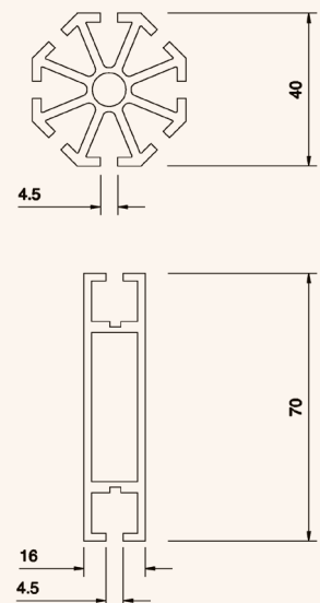
SHELL BEAM DETAIL
